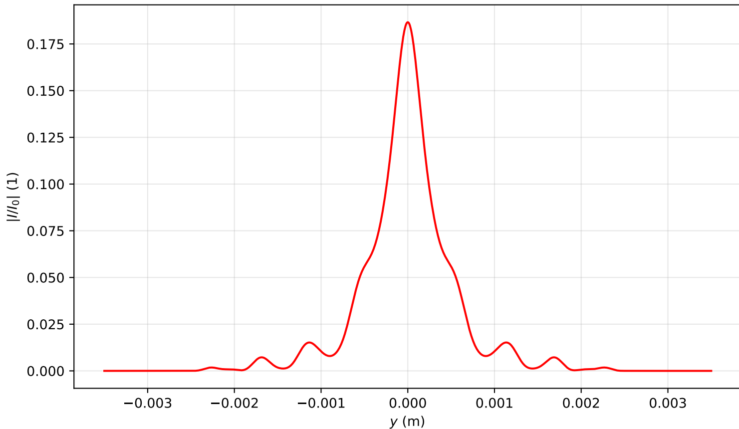
Intensity profile I(x=0, y, z=3.981)/I_0 , \text{Pin}=5.0\text{Pcr} , artificial time
